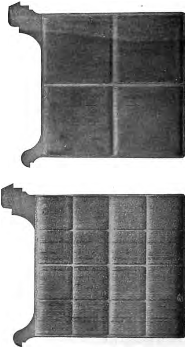
FIG. 811.—Specimen Negative Plate of a Type of the "Gould" Storage Battery, showing the result of "formation" in the changed appearance of the plate surface.
